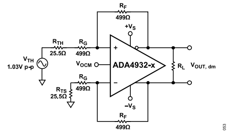
Figure 61. Thevenin Equivalent and Matched Gain Resistors
