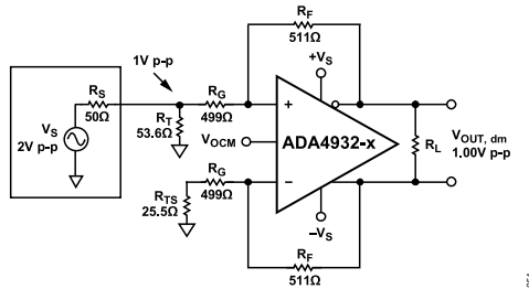
Figure 62. Terminated Single-Ended-to-Differential System with G = 2
