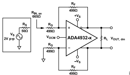
Figure 58. Calculating Single-Ended Input Impedance, R_{IN}
