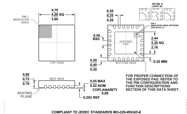
Figure 70. 24-Lead Lead Frame Chip Scale Package [LFCSP] 4 mm × 4 mm Body and 0.75 mm Package Height (CP-24-14) Dimensions shown in millimeters
