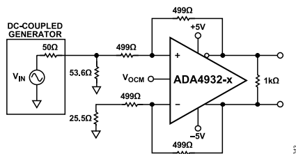
Figure 51. Equivalent Basic Test Circuit, G = 1
