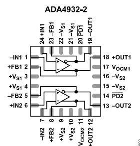
Figure 2. ADA4932-2
