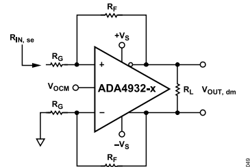
Figure 57. The ADA4932-1/ADA4932-2 with Unbalanced (Single-Ended) Input
