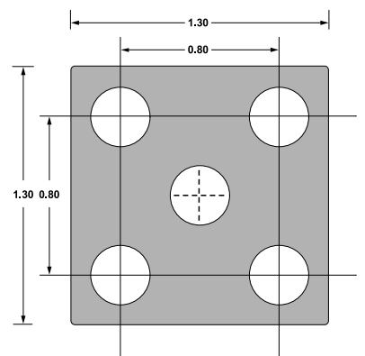
Figure 67. Recommended PCB Thermal Attach Pad Dimensions (Millimeters)
