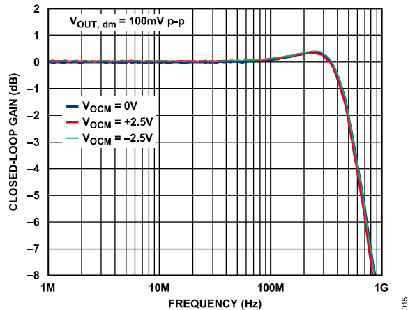
Figure 14. Small Signal Frequency Response for Various V_{OCM} Levels
