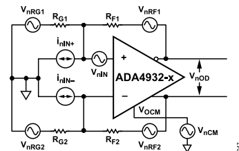
Figure 55. Noise Model
