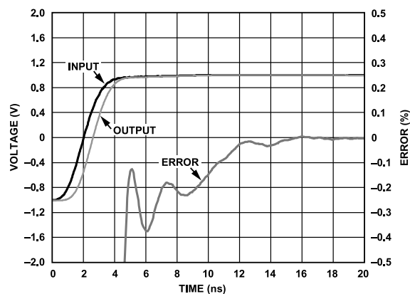
Figure 48. Settling Time
