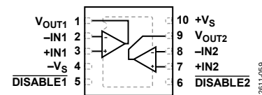
Figure 3. 10-Lead LFCSP Pin Configuration ( ADA4807-2 )
