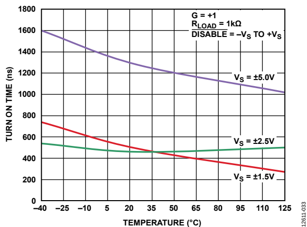
Figure 59. Turn On Time vs. Temperature and Supply
