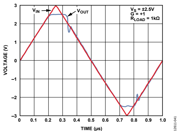
Figure 58. Input Overdrive Recovery
