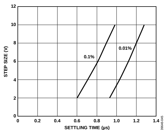
Figure 53. Negative Step Settling Time
