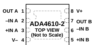
Figure 5. ADA4610-2 Pin Configuration, 8-Lead MSOP (RM Suffix)
