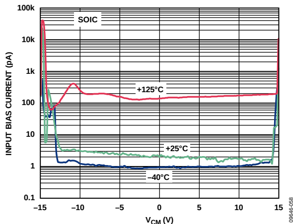
Figure 19. Input Bias Current vs. Common-Mode Input Voltage ( V_{CM} ), Three Temperatures, V_{SV} = \pm 15\text{ V} , R_L = \infty
