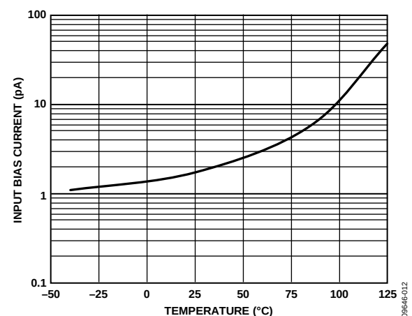
Figure 20. Input Bias Current vs. Temperature, V_{SV} = \pm 15\text{ V}
