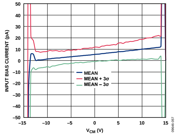
Figure 18. Input Bias Current vs. Common-Mode Input Voltage ( V_{CM} ), Mean and Three Standard Deviations, V_{SV} = \pm 15\text{ V} , R_L = \infty
