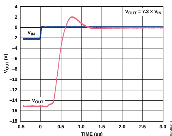
Figure 54. Negative Overload Recovery
