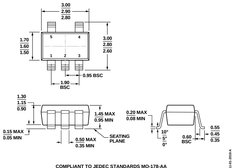
Figure 66. 5-Lead Small Outline Transistor Package [SOT-23] (RJ-5)
