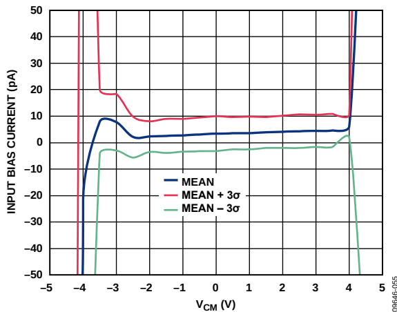
Figure 15. Input Bias Current vs. Common-Mode Input Voltage ( V_{CM} ), Mean and Three Standard Deviations, V_{SV} = \pm 5\text{ V} , R_L = \infty
