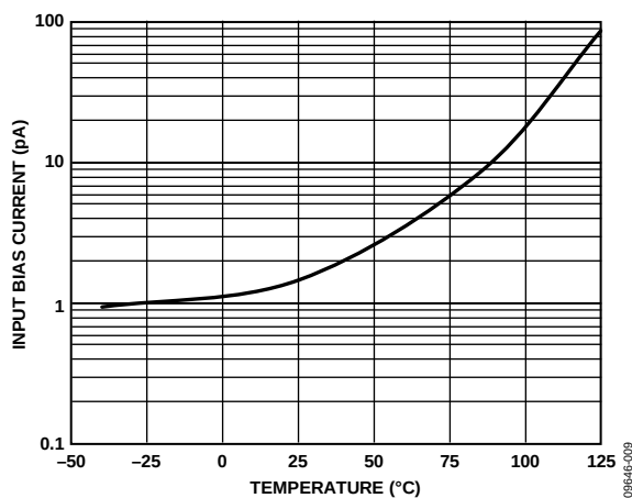
Figure 17. Input Bias Current vs. Temperature, V_{SV} = \pm 5\text{ V}
