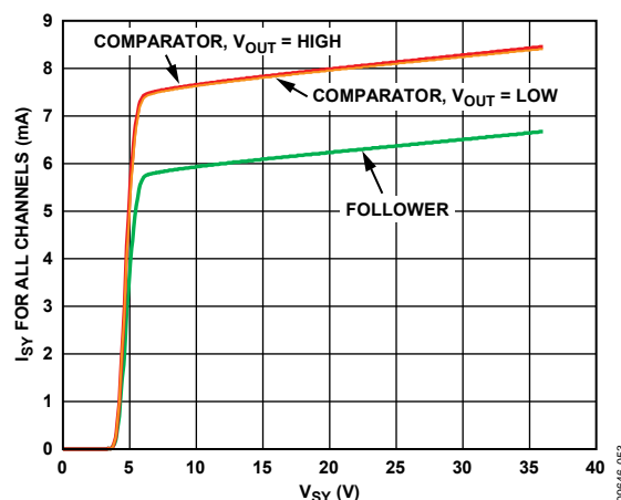
Figure 60. Supply Current ( I_{SV} ) vs. Supply Voltage ( V_{SV} ) for the ADA4610-4 Only
