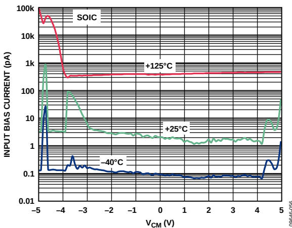
Figure 16. Input Bias Current vs. Common-Mode Input Voltage ( V_{CM} ), Three Temperatures, V_{SV} = \pm 5\text{ V} , R_L = \infty
