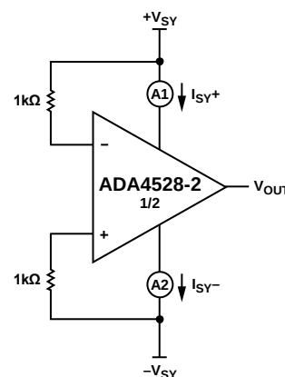
Figure 70. Comparator A
