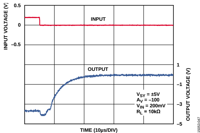
Figure 40. Negative Overload Recovery, V_{SY} = \pm 5\text{ V}
