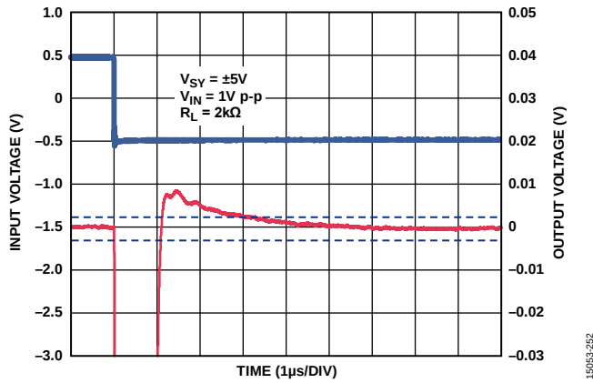
Figure 46. Negative 0.1% Settling Time, V_{SV} = \pm 5 V
