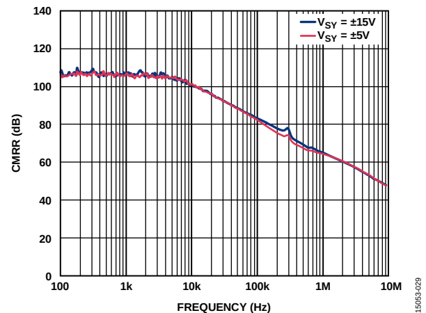
Figure 27. CMRR vs. Frequency, V_{SY} = \pm 5\text{ V} and V_{SY} = \pm 15\text{ V}
