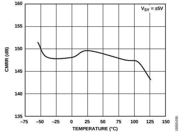
Figure 26. CMRR vs. Temperature, V_{SY} = \pm 5\text{ V}
