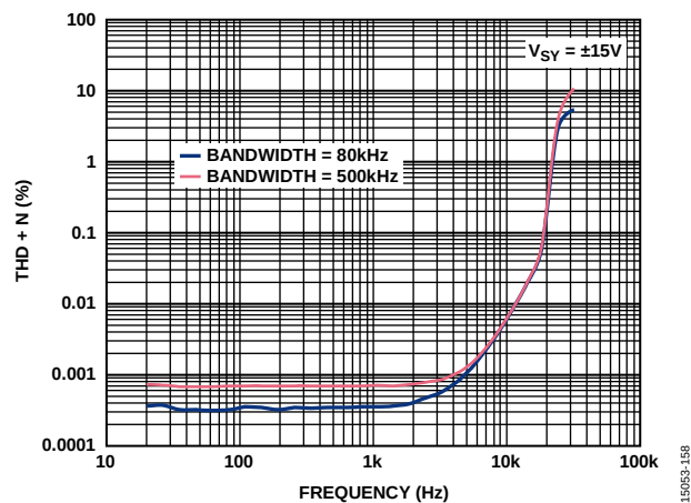
Figure 51. THD + N vs. Frequency, V_{SV} = \pm 15 V
