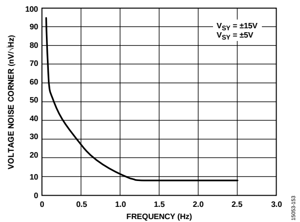
Figure 50. Voltage Noise Corner vs. Frequency, V_{SV} = \pm 15 V and V_{SV} = \pm 5 V
