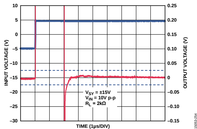
Figure 45. Positive 0.1% Settling Time, V_{SY} = \pm 15\text{ V}
