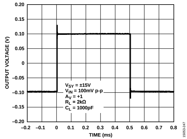
Figure 38. Small Signal Transient Response, V_{SY} = \pm 15V
