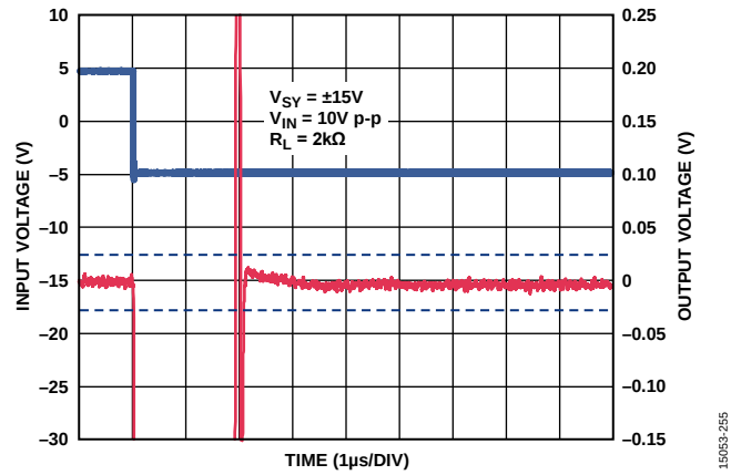
Figure 49. Negative 0.1% Settling Time, V_{SV} = \pm 15 V
