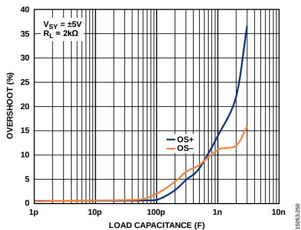
Figure 41. Small Signal Overshoot vs. Load Capacitance, V_{SY} = \pm 5\text{ V}
