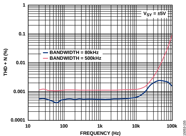
Figure 48. THD + N vs. Frequency, V_{SV} = \pm 5 V
