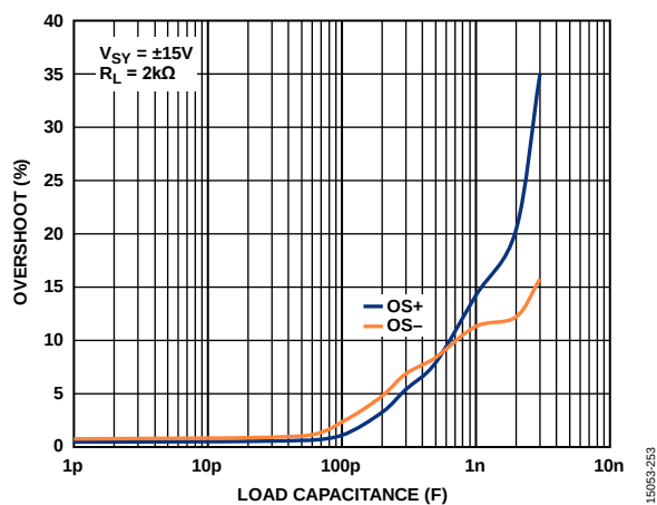
Figure 44. Small Signal Overshoot vs. Load Capacitance, V_{SY} = \pm 15\text{ V}
