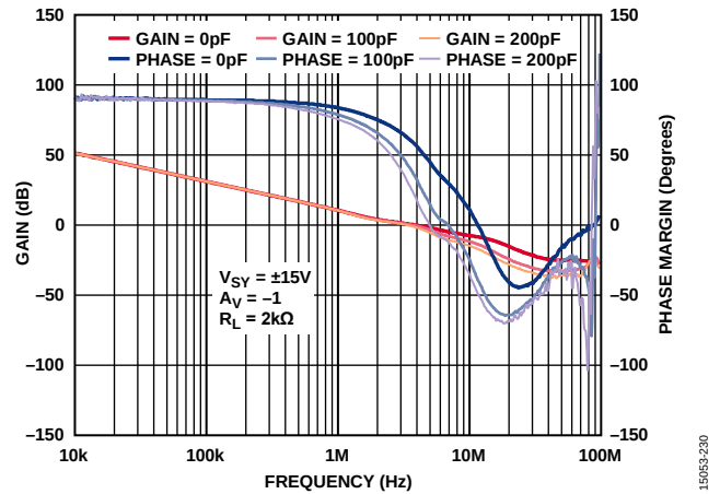
Figure 25. Open-Loop Gain and Phase Margin vs. Frequency, V_{SY} = \pm 15\text{ V}
