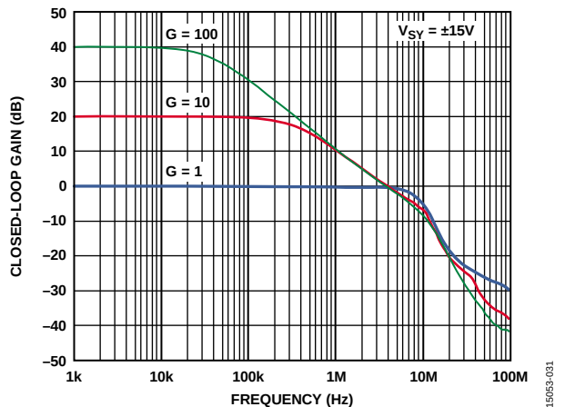
Figure 33. Closed-Loop Gain vs. Frequency, V_{SY} = \pm 15\text{ V}
