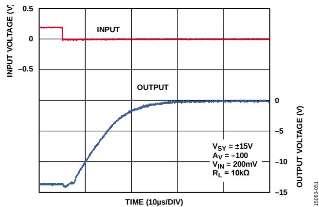
Figure 43. Negative Overload Recovery, V_{SY} = \pm 15\text{ V}
