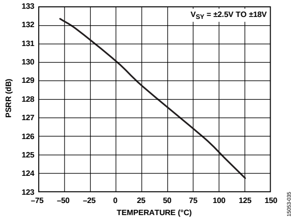
Figure 23. PSRR vs. Temperature, V_{SY} = \pm 2.5\text{ V TO } \pm 18\text{ V}
