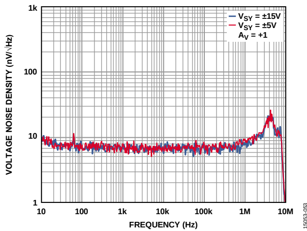
Figure 47. Voltage Noise Density vs. Frequency, V_{SV} = \pm 5 V and V_{SV} = \pm 15 V
