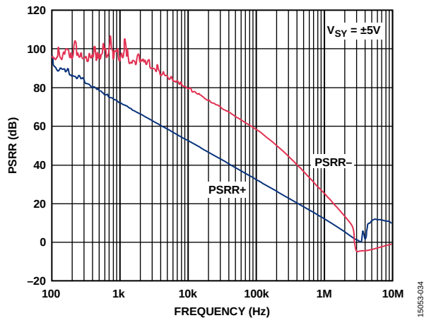
Figure 24. PSRR vs. Frequency, V_{SY} = \pm 5\text{ V}
