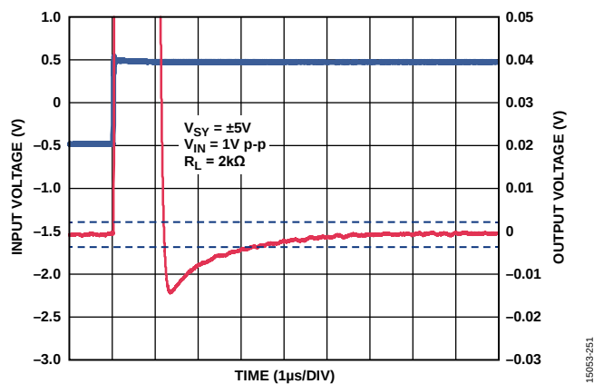
Figure 42. Positive 0.1% Settling Time, V_{SY} = \pm 5\text{ V}
