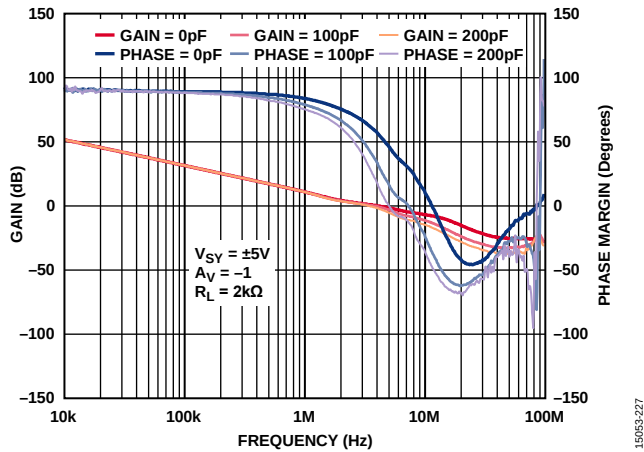
Figure 22. Open-Loop Gain and Phase Margin vs. Frequency, V_{SY} = \pm 5\text{ V}
