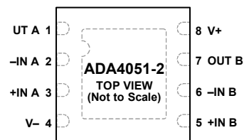
Figure 3. 8-Lead MSOP (RM-8)
