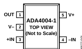
Figure 1. 5-Lead SOT (RJ-5)
