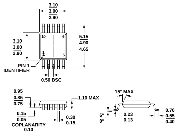
Figure 23. 10-Lead Mini Small Outline Package [MSOP] (RM-10) Dimensions shown in millimeters
