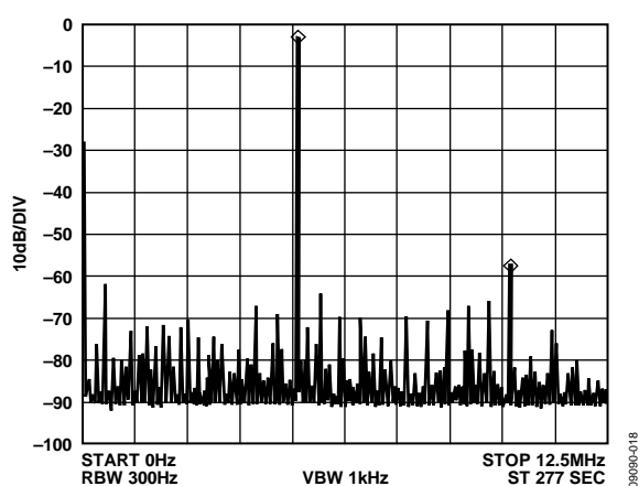
Figure 18. f_{\text{MCLK}} = 25 \text{ MHz} , f_{\text{OUT}} = 5.1 \text{ MHz} , Frequency Word = 0x34395810
