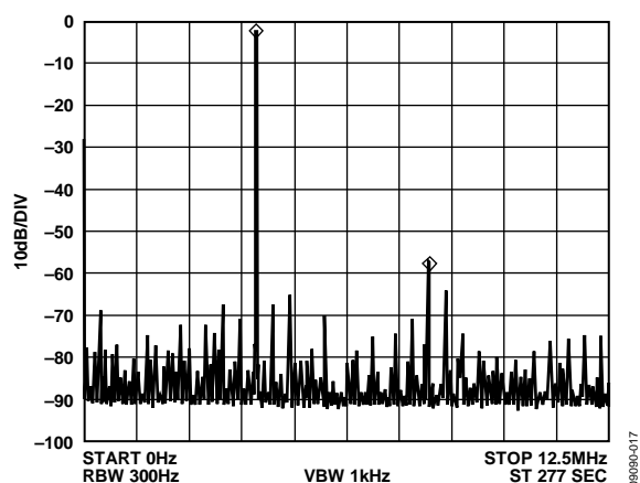
Figure 17. f_{\text{MCLK}} = 25 \text{ MHz} , f_{\text{OUT}} = 4.1 \text{ MHz} , Frequency Word = 0x29FBE76D
