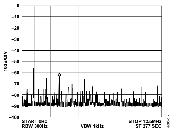
Figure 14. f_{\text{MCLK}} = 25 \text{ MHz} , f_{\text{OUT}} = 1.1 \text{ MHz} , Frequency Word = 0xB439581
