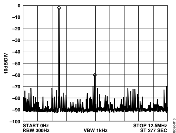
Figure 16. f_{\text{MCLK}} = 25 \text{ MHz} , f_{\text{OUT}} = 3.1 \text{ MHz} , Frequency Word = 0x1FBE76C9
