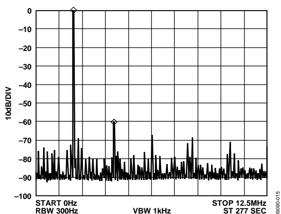
Figure 15. f_{\text{MCLK}} = 25 \text{ MHz} , f_{\text{OUT}} = 2.1 \text{ MHz} , Frequency Word = 0x15810625
