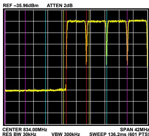
Figure 43. 4-Channel QAM ACLR, f_{OUT} = 840 MHz, Temperature = 25°C, Sum Scale = 20, Full-Scale Current = 25 mA, Span = 42 MHz, Channel 1
