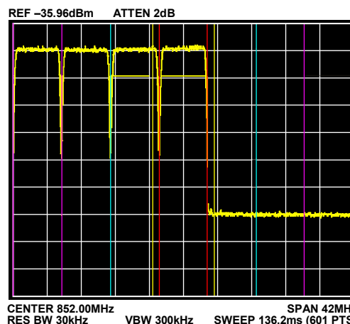
Figure 45. 4-Channel QAM ACLR, f_{OUT} = 840 MHz, Temperature = 25°C, Sum Scale = 20, Full-Scale Current = 25 mA, Span = 42 MHz, Channel 4
