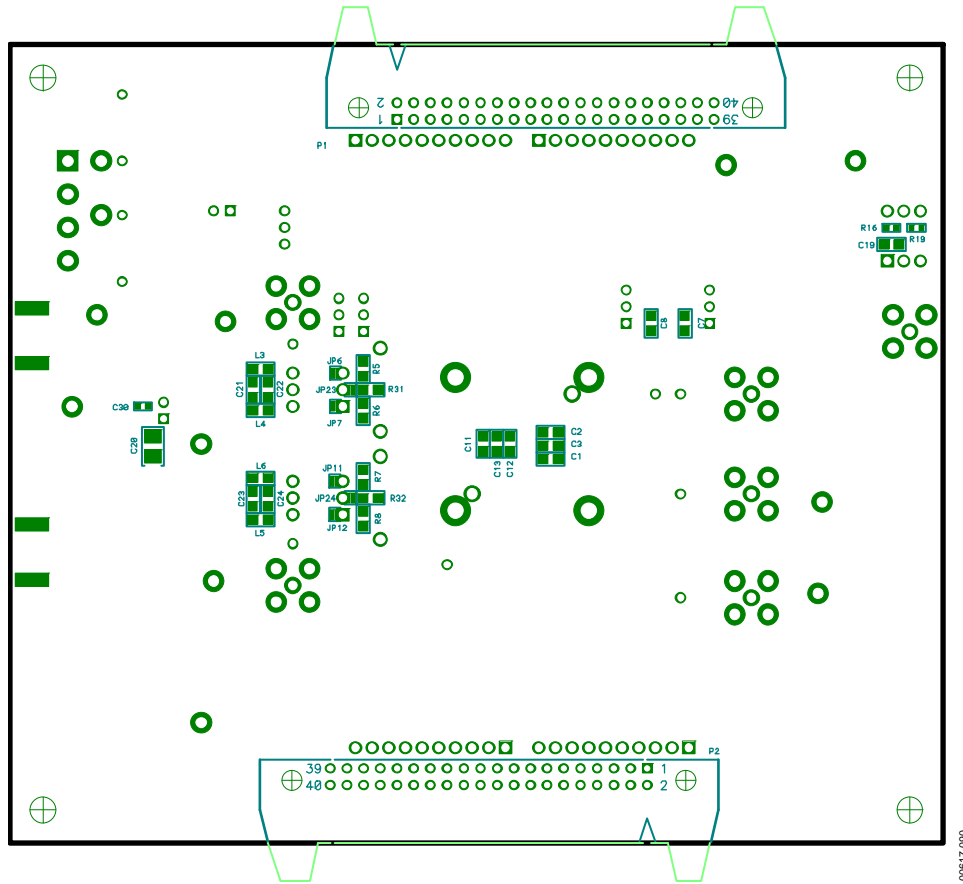
Figure 93. Assembly, Bottom Side
