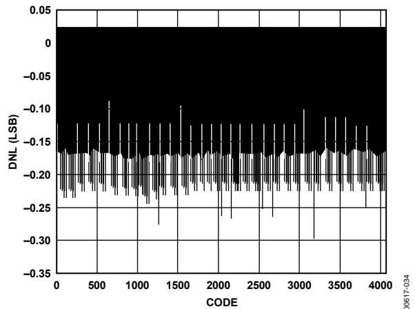
Figure 34. Typical DNL
