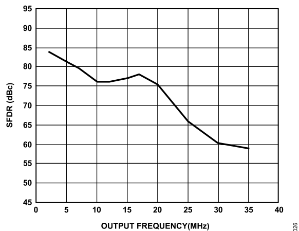
Figure 29. SFDR vs. f_{OUT} at 80 MSPS
