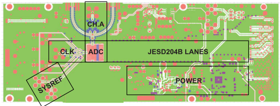
Figure 128. Recommended PCB Layout for the AD9699
