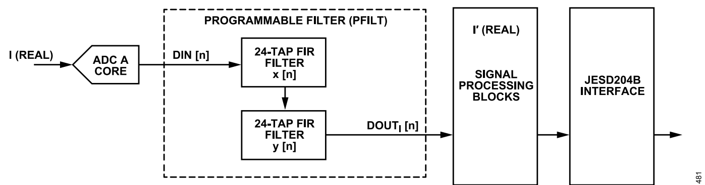
Figure 80. Real, Two Cascaded, 24-Tap Filter Configuration
