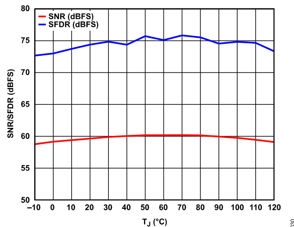
Figure 33. SNR/SFDR vs. T_J , f_{IN} = 950 MHz, A_{IN} = -9 dBFS
