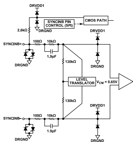
Figure 45. SYNCINB± Inputs
