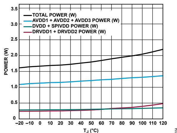
Figure 34. Power vs. T_J , f_{IN} = 950 MHz
