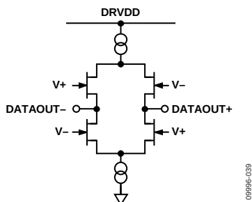
Figure 42. Equivalent LVDS Output Circuit
