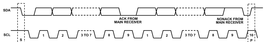
Figure 56. Data Transfer Process (Main Read Mode, 2-Byte Transfer)
