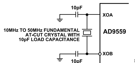
Figure 33. System Clock Input (XOA/XOB) in Crystal Mode (The recommended C_{LOAD} = 10 pF is shown. The values of 10 pF shunt capacitors shown here should equal the C_{LOAD} of the crystal.)
