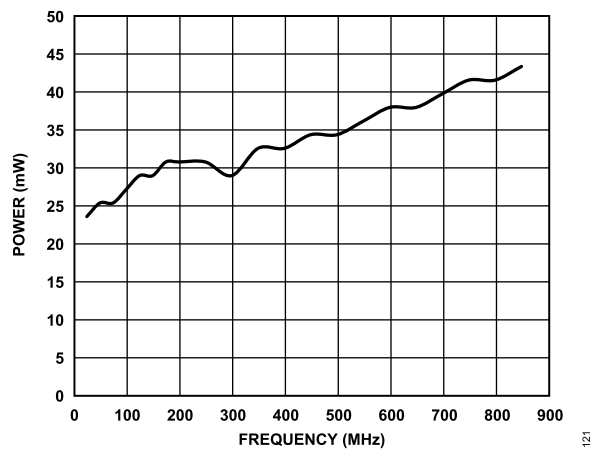
Figure 21. Power Consumption vs. Frequency, LVDS Mode on Output Driver Power Supply Only (Pin 17, Pin 21, Pin 34, and Pin 38)
