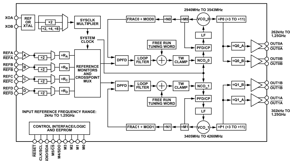
Figure 35. Detailed Block Diagram
