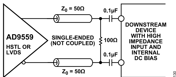
Figure 30. AC-Coupled LVDS or HSTL Output Driver (100 \Omega resistor can be placed on either side of decoupling capacitors and should be as close to the destination receiver as possible.)
