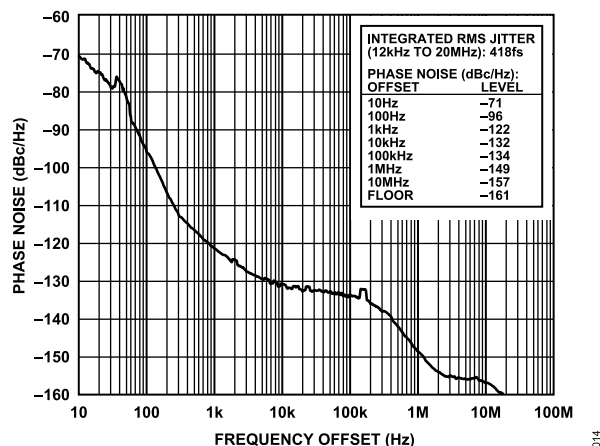
Figure 15. Absolute Phase Noise (Output Driver = 1.8V CMOS), f_R = 2 kHz, f_{OUT} = 70.656 MHz, DPLL Loop BW = 10 Hz, f_{SYS} = 19.2 MHz TCXO
