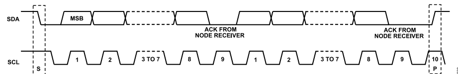
Figure 55. Data Transfer Process (Main Write Mode, 2-Byte Transfer)
