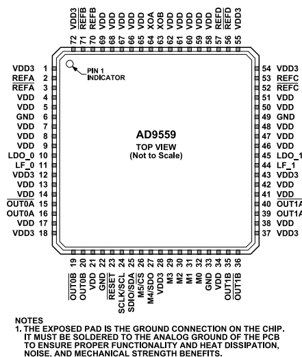
Figure 2. Pin Configuration
