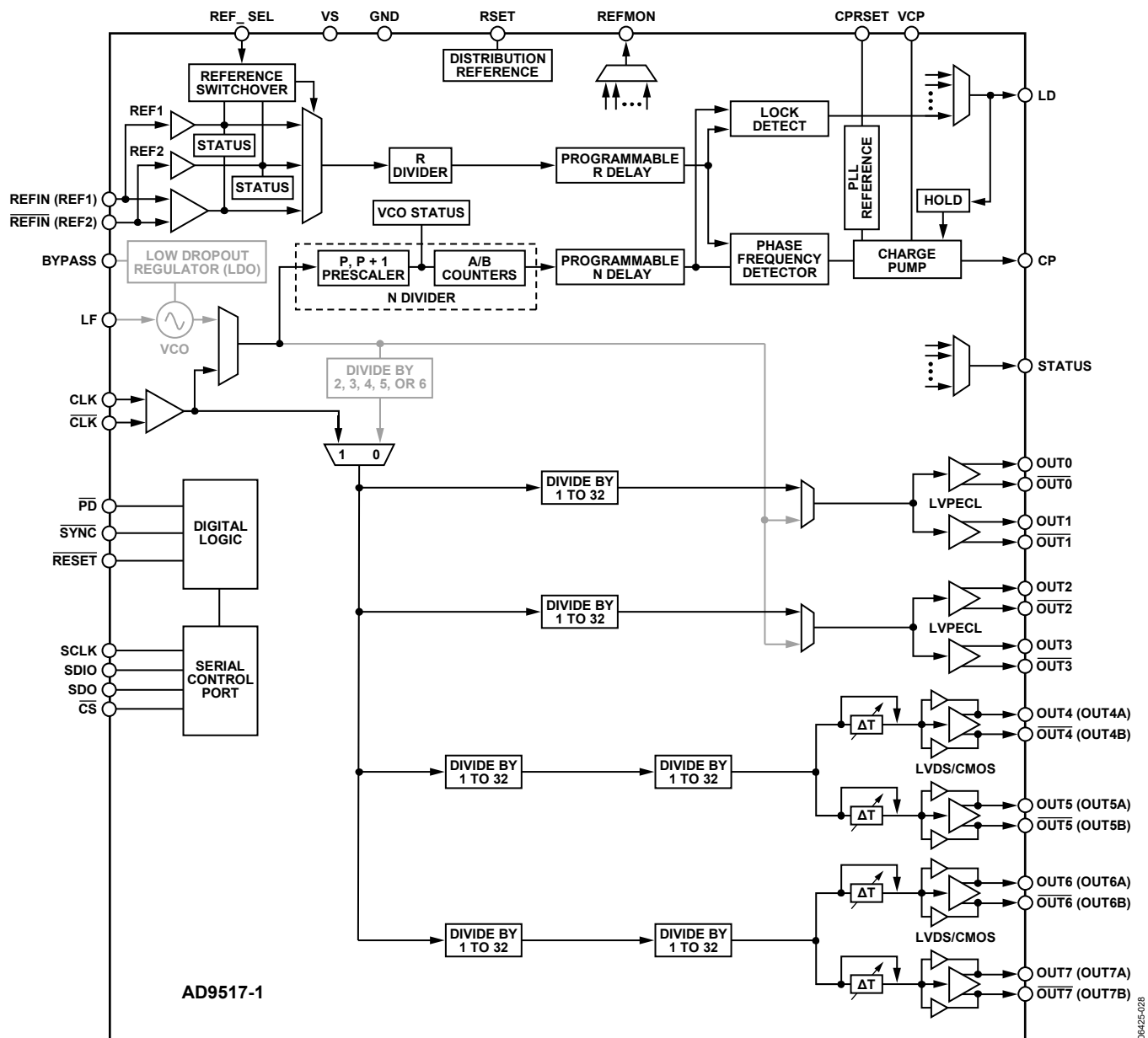
Figure 45. Clock Distribution or External VCO &lt; 1600 MHz
