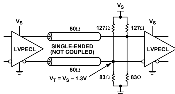
Figure 35. LVPECL Far-End Termination
