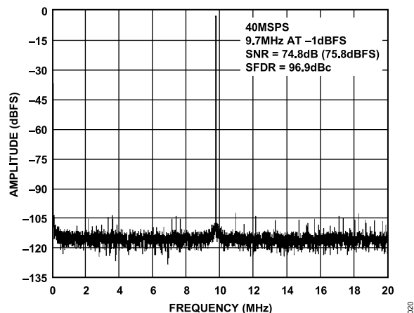
Figure 21. Single-Tone 16k FFT with f_{IN} = 9.7 MHz, f_{SAMPLE} = 40 MSPS
