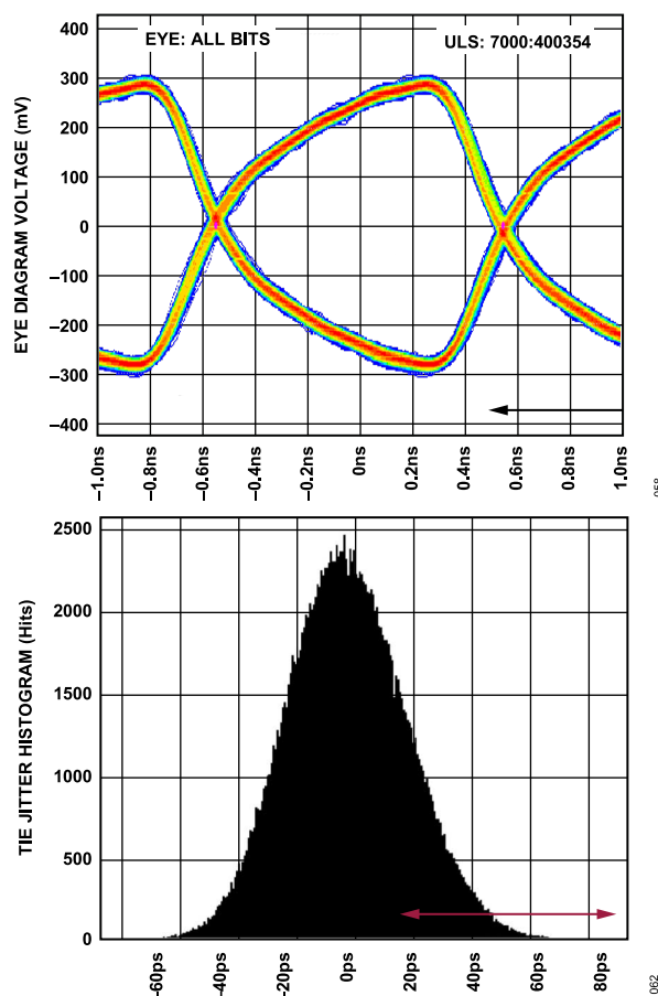
Figure 59. Data Eye for LVDS Outputs in ANSI-644 Mode with Trace Lengths Less Than 24 Inches on Standard FR-4, External 100 \Omega Far Termination Only
