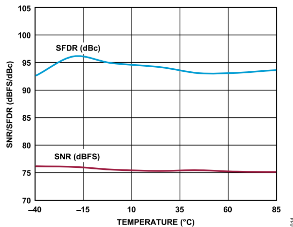
Figure 15. SNR/SFDR vs. Temperature, f_{IN} = 9.7 MHz, f_{SAMPLE} = 65 MSPS
