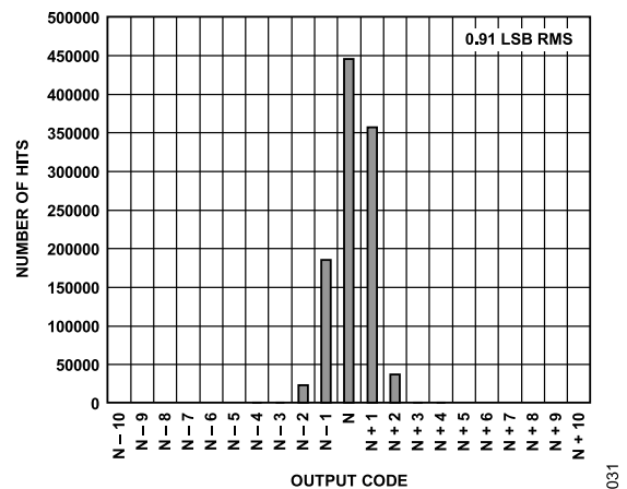
Figure 32. Input-Referred Noise Histogram, f_{SAMPLE} = 40 MSPS
