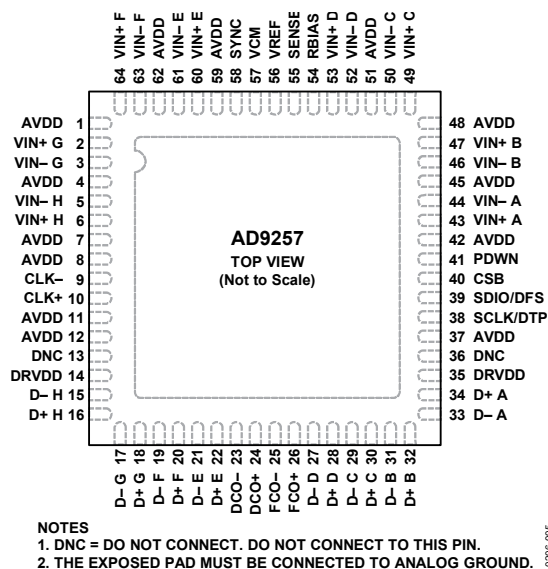
Figure 5. Pin Configuration, Top View
