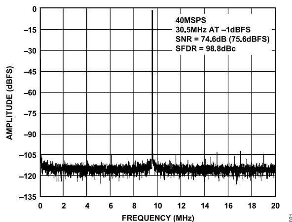
Figure 22. Single-Tone 16k FFT with f_{IN} = 30.5 MHz, f_{SAMPLE} = 40 MSPS, CLK Divider = 8
