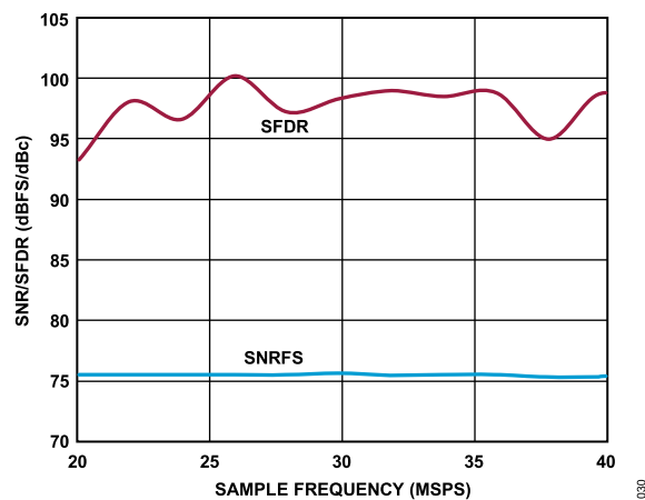
Figure 31. SNR/SFDR vs. Encode, f_{IN} = 30.5 MHz, CLK Divider = 4
