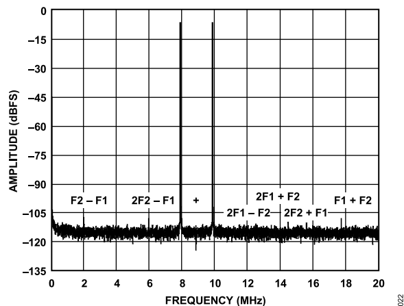
Figure 23. Two-Tone 16k FFT with f_{IN1} = 8 MHz and f_{IN2} = 10 MHz, f_{SAMPLE} = 40 MSPS
