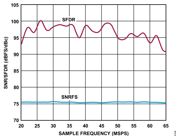
Figure 17. SNR/SFDR vs. Encode, f_{IN} = 30.5 MHz, CLK Divider = 4
