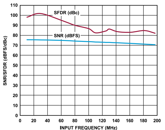
Figure 16. SNR/SFDR vs. f_{IN} , f_{SAMPLE} = 65 MSPS
