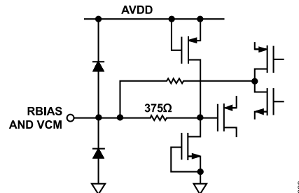
Figure 40. Equivalent RBIAS, VCM Circuit
