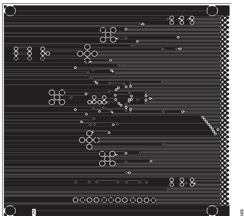
Figure 49. Ground Plane
