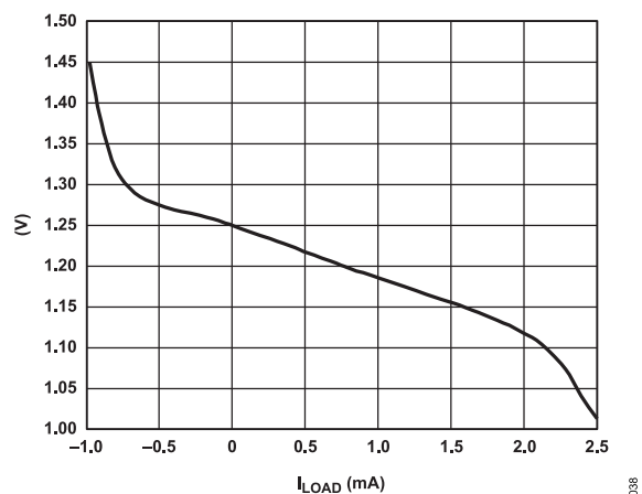
Figure 38. V_{REF} vs. I_{LOAD}
