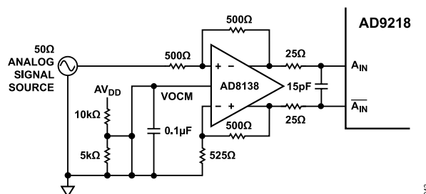
Figure 43. Using the AD8138 to Drive the AD9218
