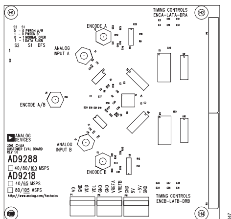
Figure 47. Top Silkscreen
