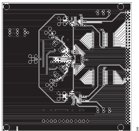
Figure 48. Top Routing
