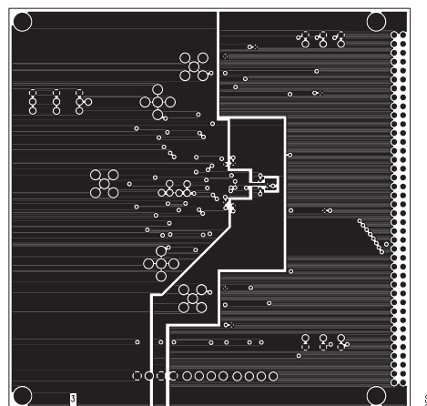
Figure 50. Split Power Plane
