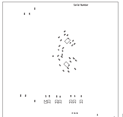
Figure 52. Bottom Silkscreen
