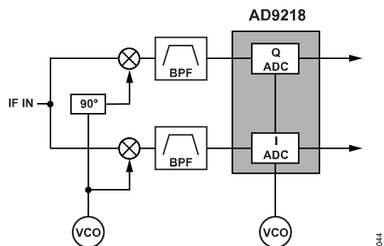
Figure 44. Typical I/Q Demodulation Scheme
