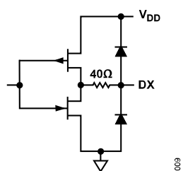
Figure 9. Digital Output Stage
