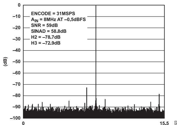
Figure 23. FFT: FS = 31 MSPS, A_{IN} = 8\text{ MHz @ } -0.5\text{ dBFS} , Differential, with AD8138 Driving ADC Inputs, 1 V p-p Input Range
