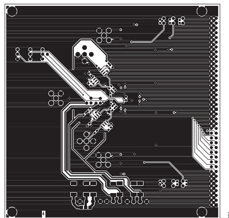
Figure 51. Bottom Routing
