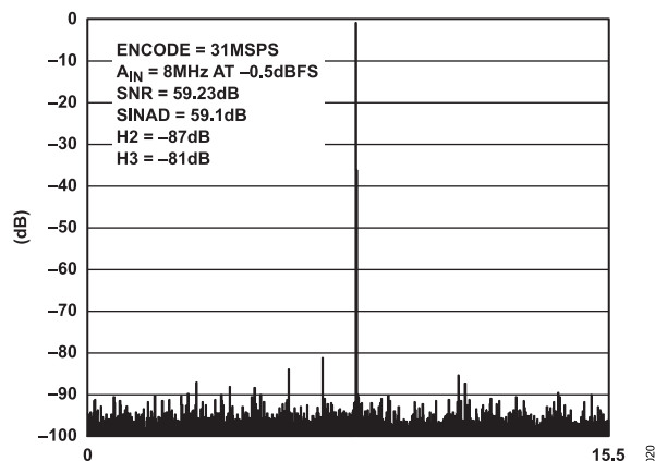
Figure 20. FFT: FS = 31 MSPS, A_{IN} = 8\text{ MHz @ } -0.5\text{ dBFS} , Differential, 1 V p-p Input Range
