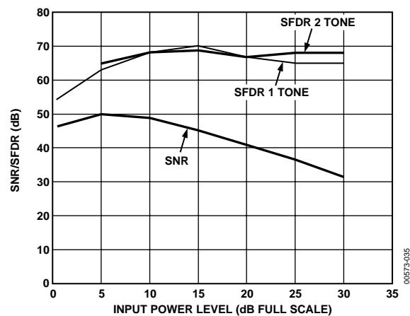
Figure 35. SNR/SFDR for IF @ 130 MHz (Clock = 40 MSPS)
