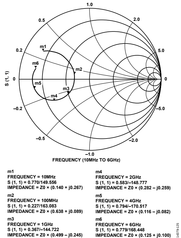
Figure 194. Simulated Smith Chart Showing the DAC Output Impedance ( Z_0 = 100 \Omega )
