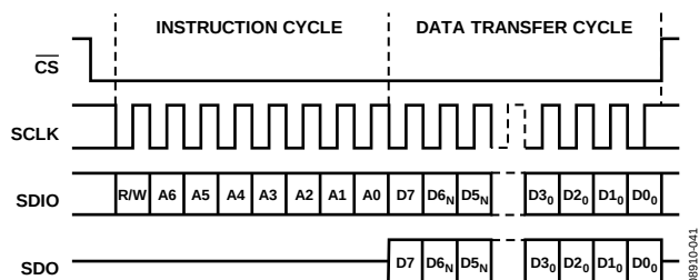
Figure 41. Serial Register Interface Timing MSB First
