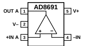
Figure 2. 5-Lead SC70
