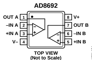
Figure 3. 8-Lead SOIC and 8-Lead MSOP
