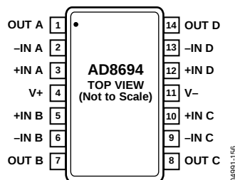
Figure 4. 14-Lead SOIC and 14-Lead TSSOP
