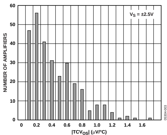
Figure 5. |TCV_{OS}| Distribution
