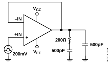
Figure 55. Snubber Network
