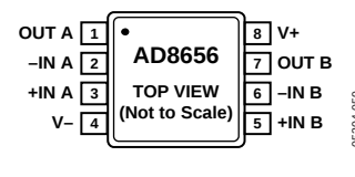
Figure 2. AD8656 8-Lead MSOP (RM-8) 8-Lead SOIC (R-8)
