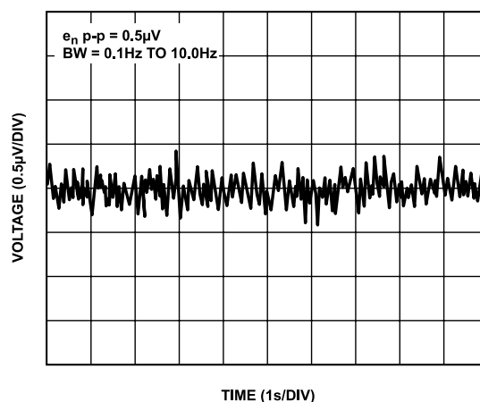
Figure 50. AD8628 Peak-to-Peak Noise
