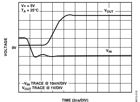
Figure 21. Rising Edge Response
