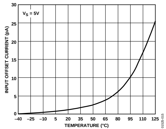
Figure 15. Input Offset Current vs. Temperature
