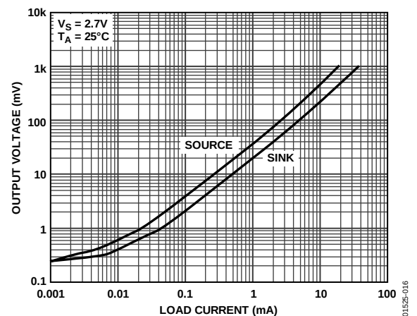
Figure 16. Output Voltage to Supply Rail vs. Load Current
