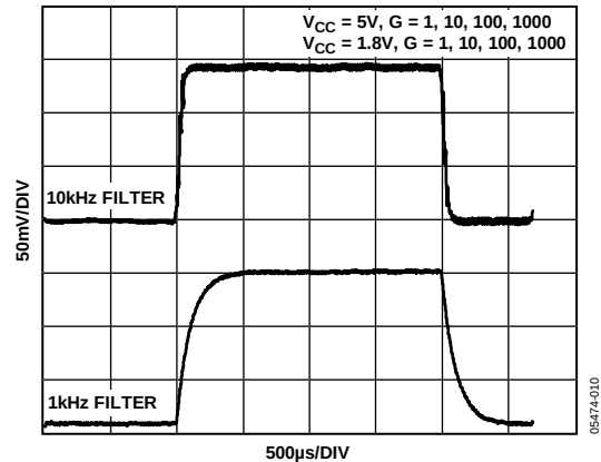
Figure 9. Small Signal Step Response
