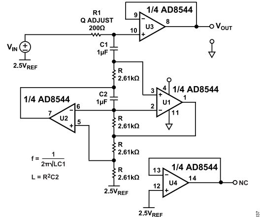
Figure 38. FDNR 60 Hz Notch Filter with Output Buffer
