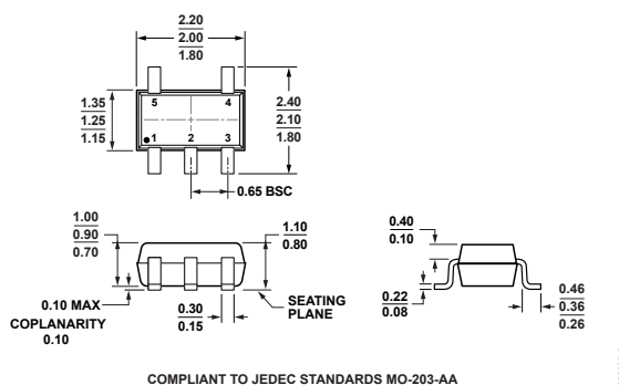
Figure 43. 5-Lead Thin Shrink Small Outline Transistor Package [SC70] (KS-5) Dimensions shown in millimeters
