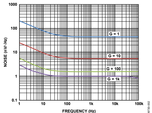
Figure 2. RTI Voltage Noise Spectral Density vs. Frequency
