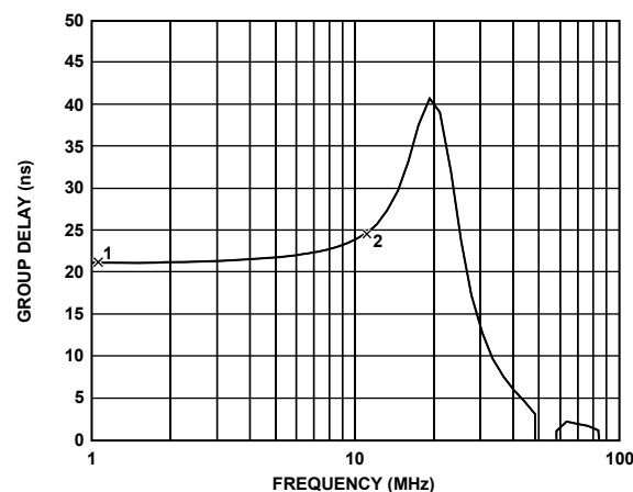
Figure 59. Baseband Filter Group Delay
