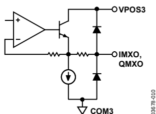
Figure 10. Circuit H
