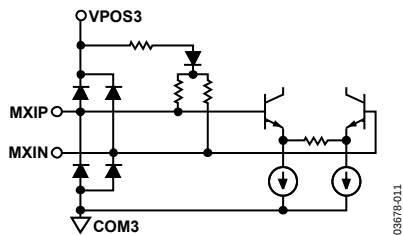
Figure 11. Circuit I
