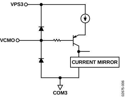
Figure 38. Circuit C
