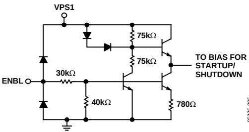
Figure 5. Circuit C
