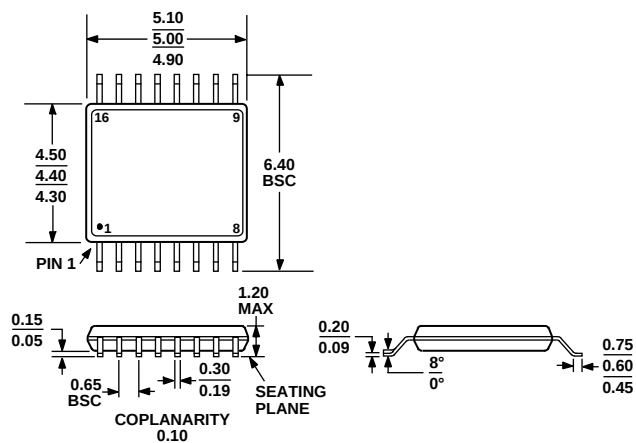
Figure 37.16. 16-Lead Thin Shrink Small Outline Package [TSSOP] (RU-16)
