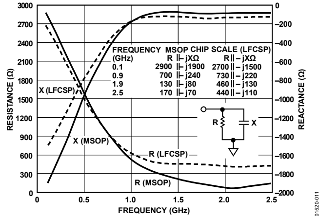
Figure 12. Input Impedance
