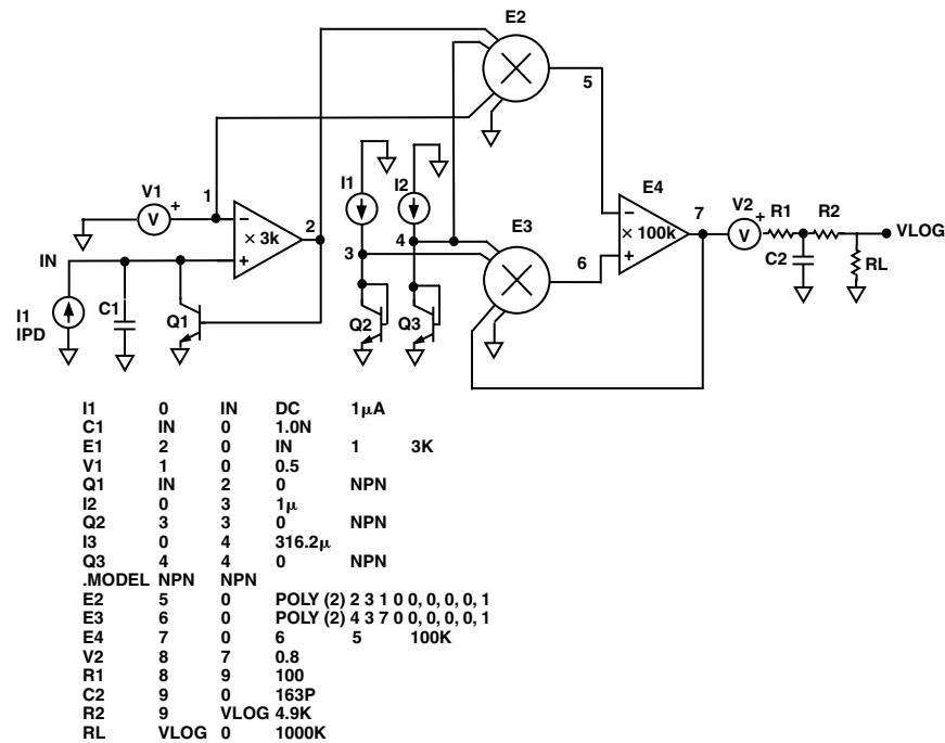
Figure 12. Basic Macromodel
