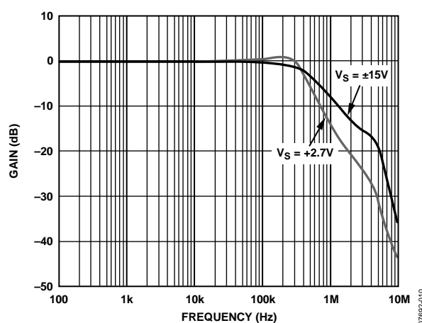
Figure 13. Gain vs. Frequency, V_S = \pm 15\text{ V} , \pm 2.7\text{ V}
