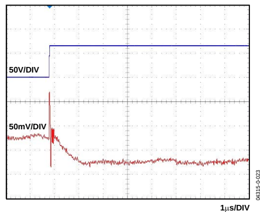
Figure 12. Common-Mode Response
