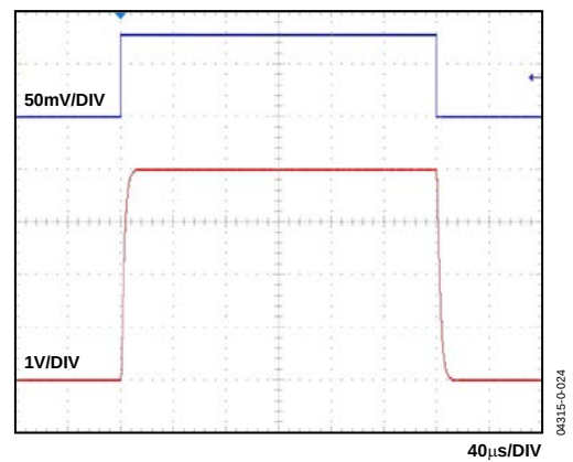
Figure 8. Rise/Fall Time
