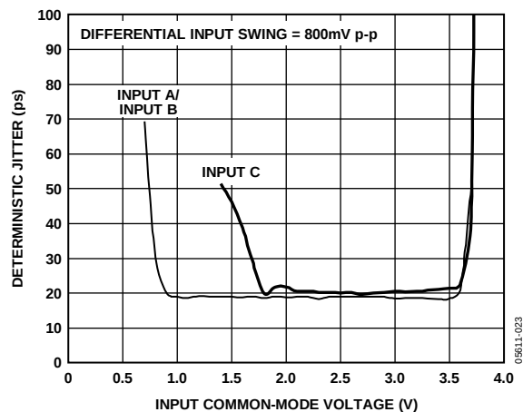
Figure 25. Deterministic Jitter vs. Input Common-Mode Voltage
