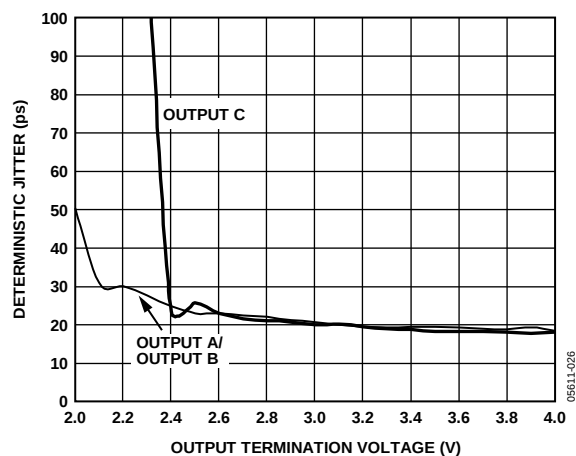
Figure 26. Deterministic Jitter vs. Output Termination Voltage
