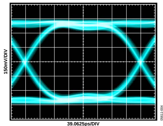
Figure 4. Output Port B Eye Diagram, 3.2 Gbps, Input Port B or Input Port C
