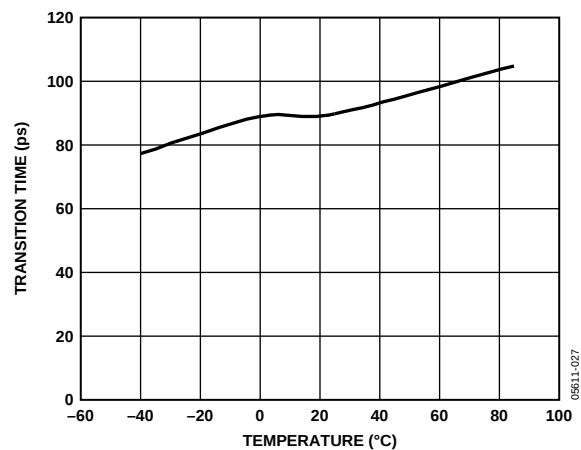
Figure 28. Transition Time vs. Temperature,
