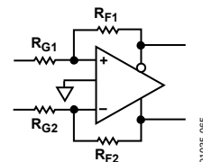
Figure 67. Typical Four-Resistor Feedback Circuit
