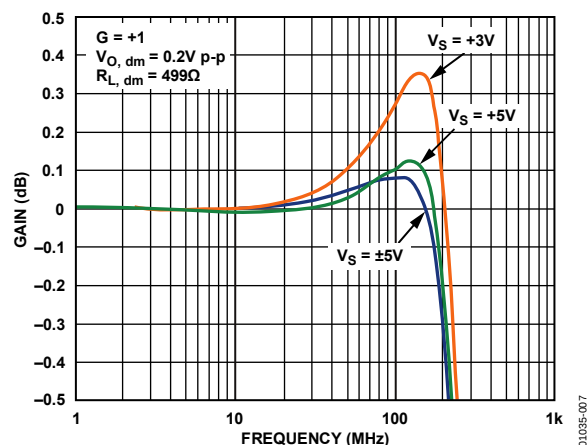
Figure 6. 0.1 dB Flatness vs. Frequency; C_F = 0 pF (See Figure 56)
