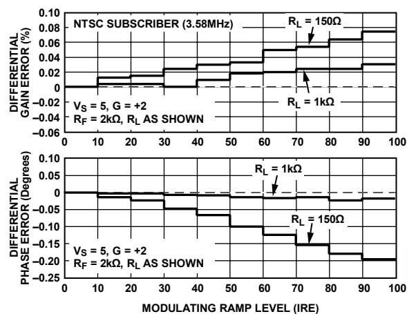
Figure 14. Differential Gain and Phase Errors
