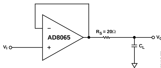
Figure 57. Output Isolation Resistor
