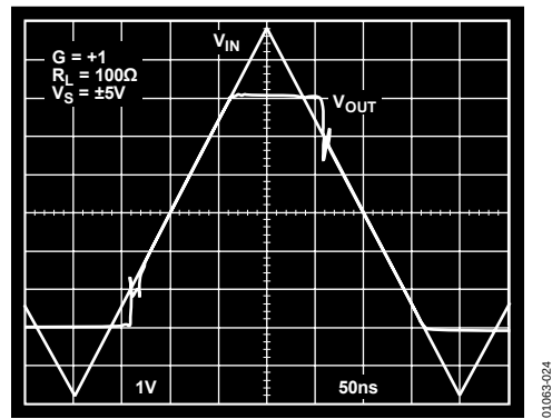
Figure 22. Overload Recovery
