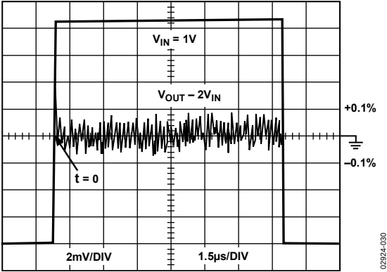
Figure 30. Long-Term Settling Time
