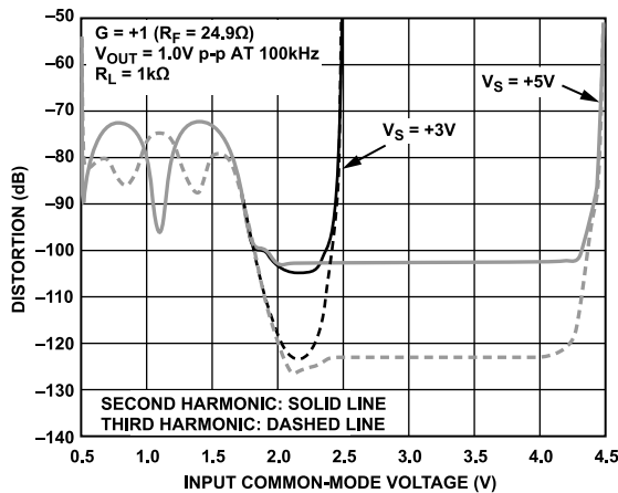
Figure 27. Harmonic Distortion vs. Input Common-Mode Voltage, \overline{DISABLE}/SELECT = High
