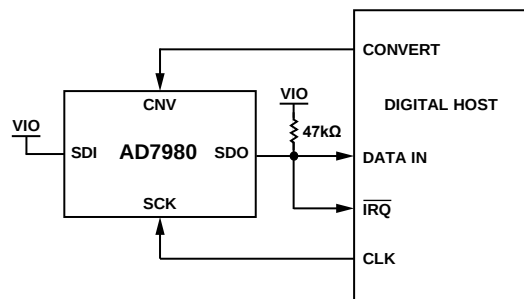
Figure 32. 3-Wire \overline{\text{CS}} Mode with Busy Indicator Connection Diagram (SDI High)
