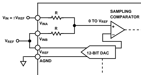
Figure 5. \pm V_{\text{REF}} Bipolar Input Configuration
