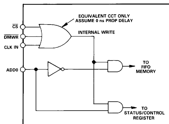
Figure 8. \overline{\text{DMWR}} Internal Logic
