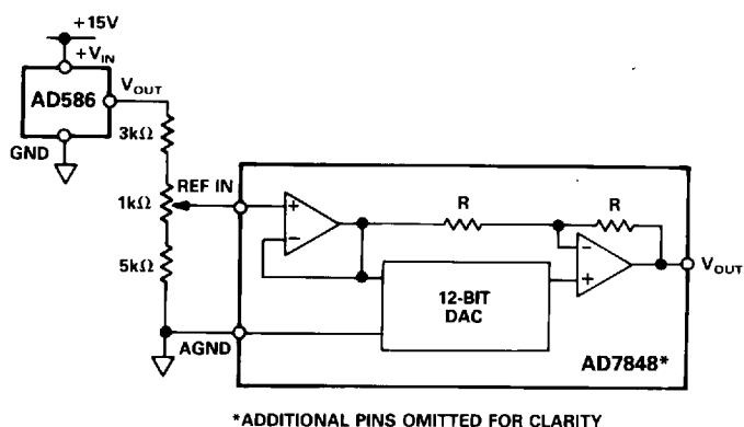
Figure 5. AD586 Driving AD7848 REF IN
