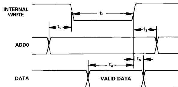
Figure 9. AD7848 Write Operation
