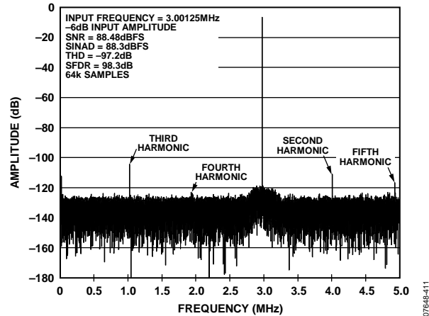
Figure 10. FFT, 3 MHz, -6 dB Input Tone, Wide View
