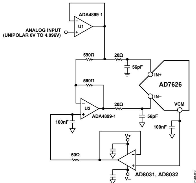
Figure 32. Single-Ended to Differential Driver Circuit Using ADA4899-1
