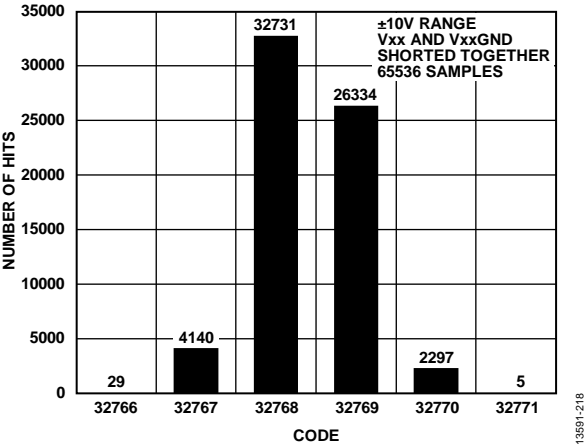
Figure 18. DC Histogram of Codes at Code Center, ±10 V Range
