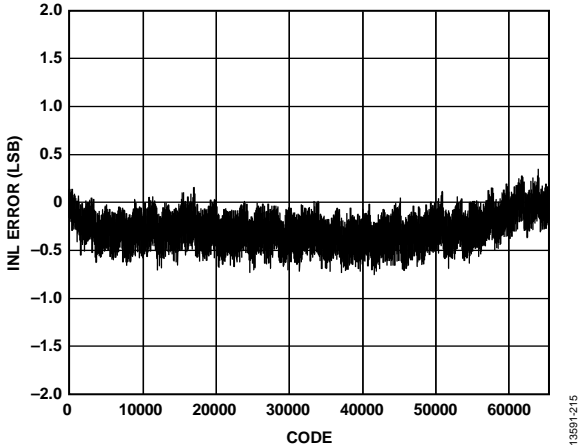
Figure 15. Typical INL Error, ±5 V Range
