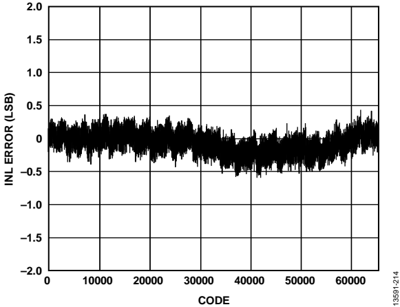
Figure 14. Typical INL Error, ±10 V Range
