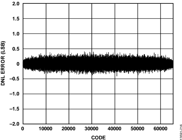
Figure 16. Typical DNL Error, ±10 V Range
