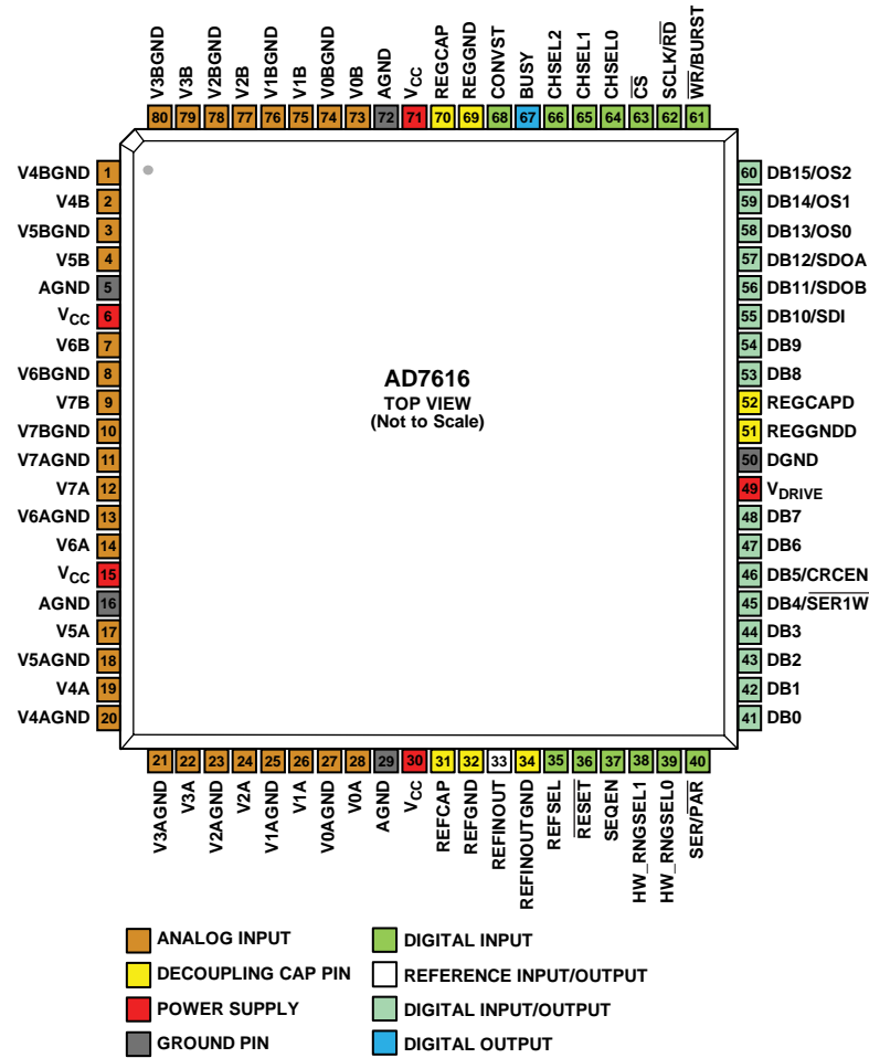
Figure 7. Pin Configuration
