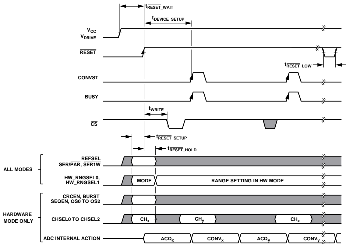
Figure 3. Reset Timing
