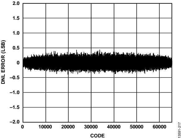
Figure 17. Typical DNL Error, ±5 V Range
