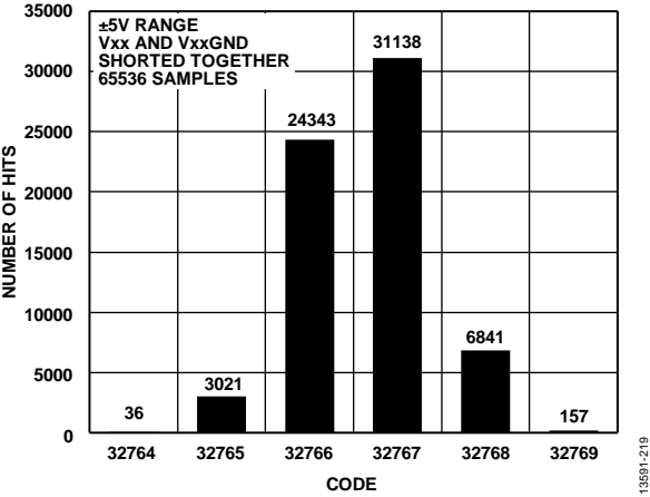
Figure 19. DC Histogram of Codes at Code Center, ±5 V Range
